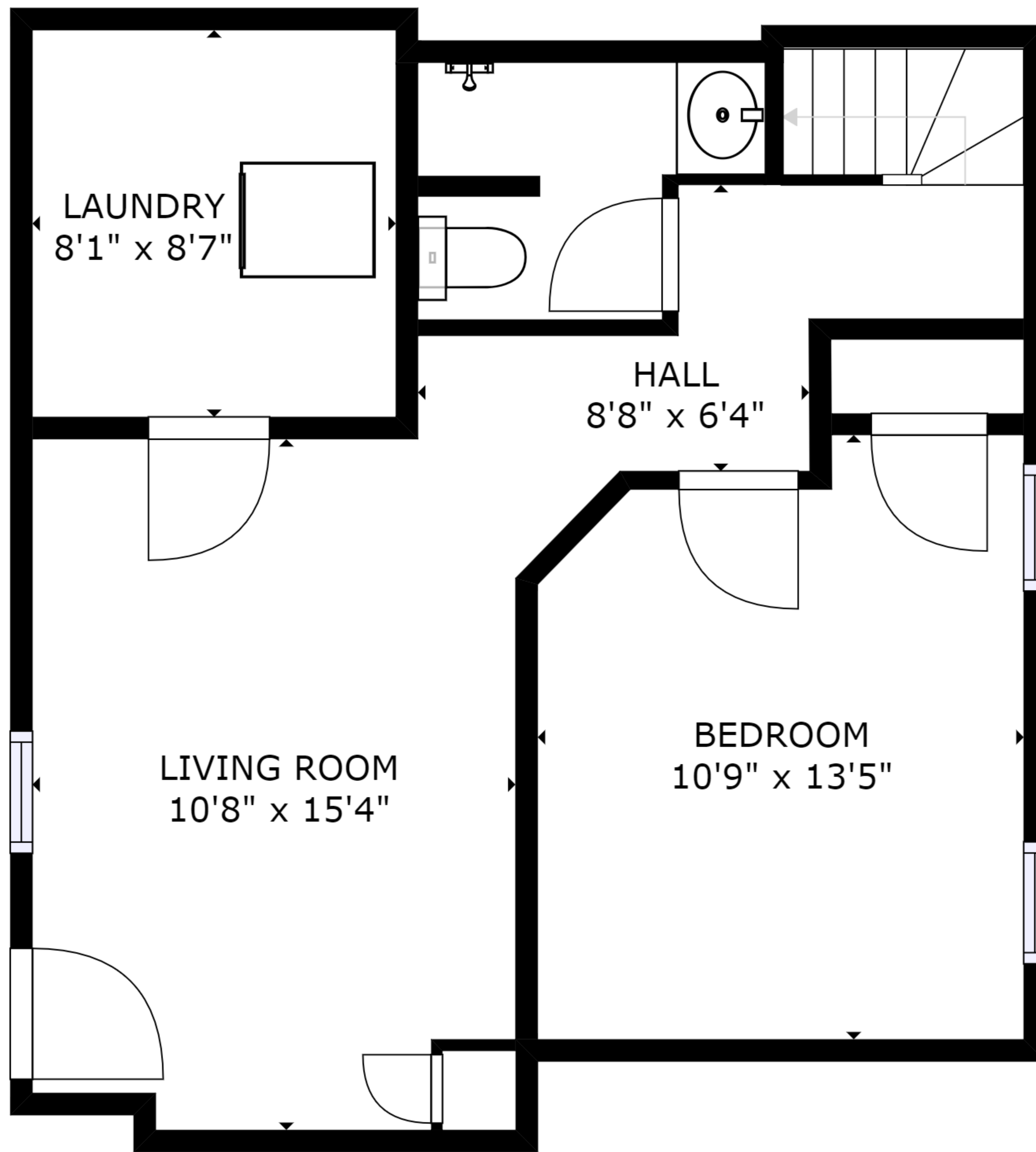
FLOOR 1
